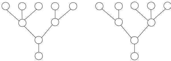
Fig. 1.2. Two different embeddings of a tree
