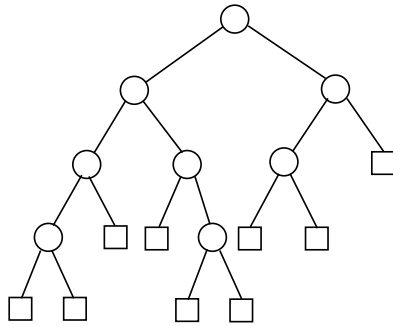
Fig. 1.5. Binary tree
